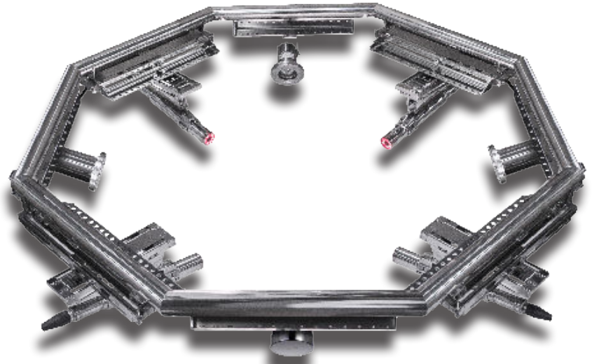
360 Fuel Inspection System Camera Ring
